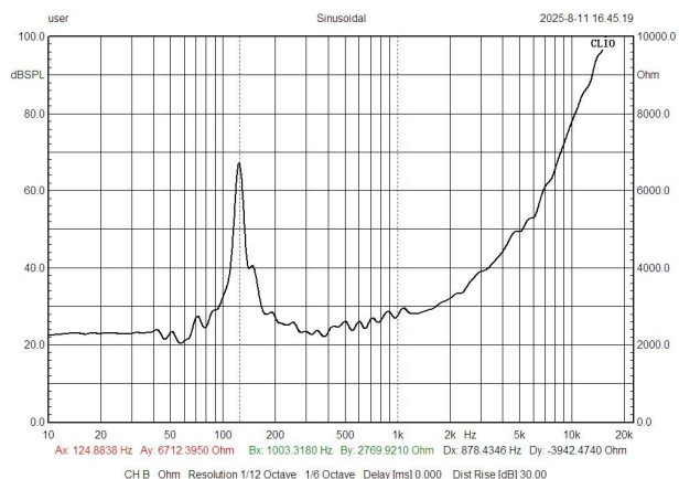
IMPEDANCE
